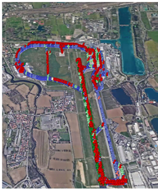
ZDR6020 Retroreflection results from airports in Europe (left) and Middle East (right) superimposed on maps. The green/red/blue colours indicate different retroreflectivity ranges.
