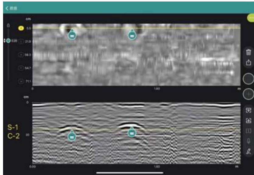
Radar 3D image slice view of a termite nest (Upper Half) and radar line scan markers (Lower Half)
