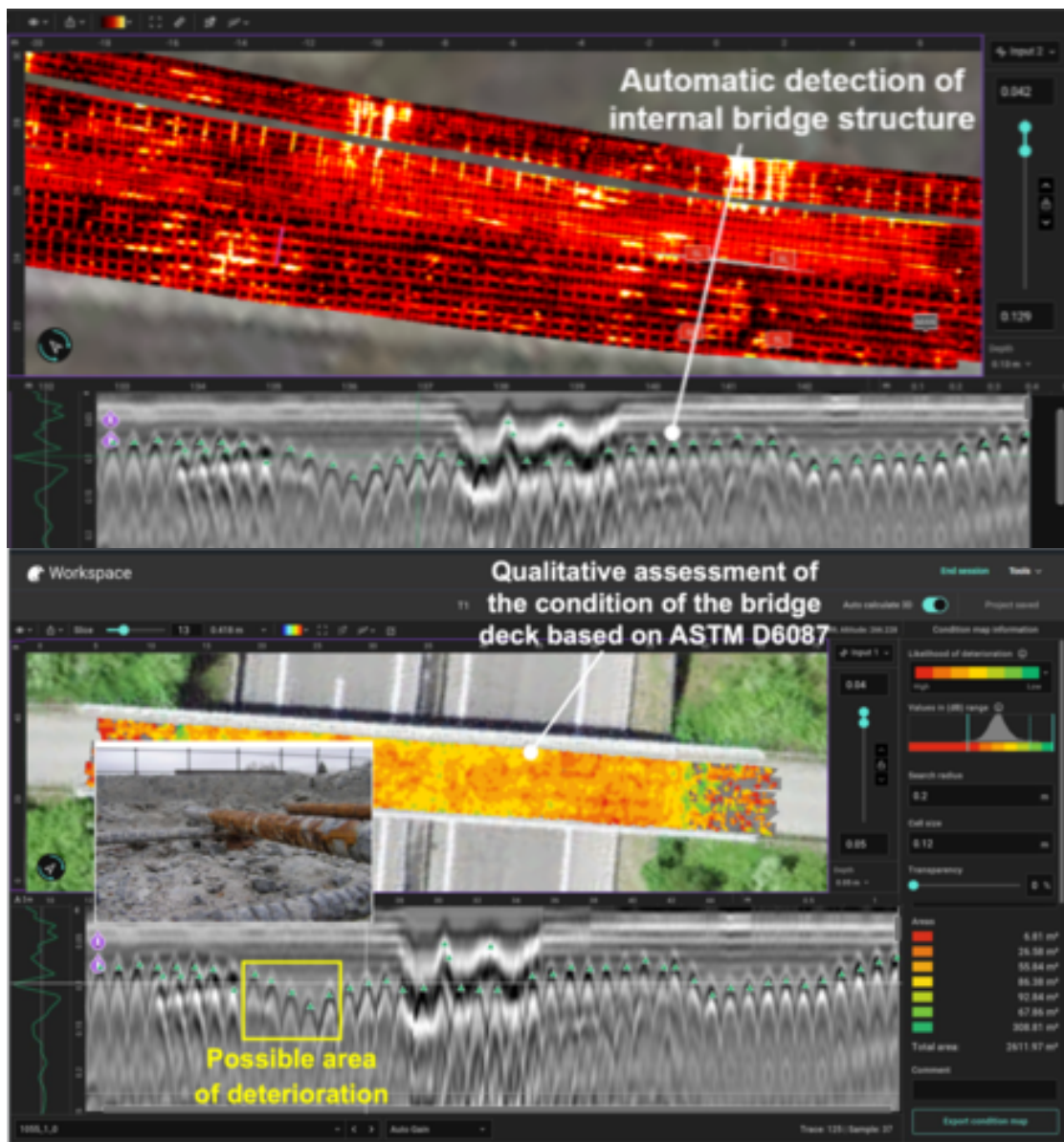
GPR Insights software showing Condition Map of bridge deck
