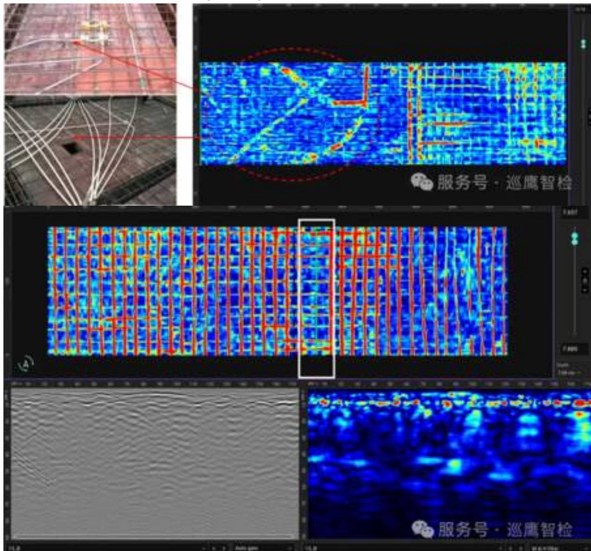
Beam body signal diagram
